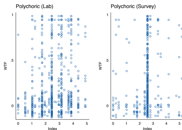
Figure D5: Scatterplot of willingness to pay and household decision making index
