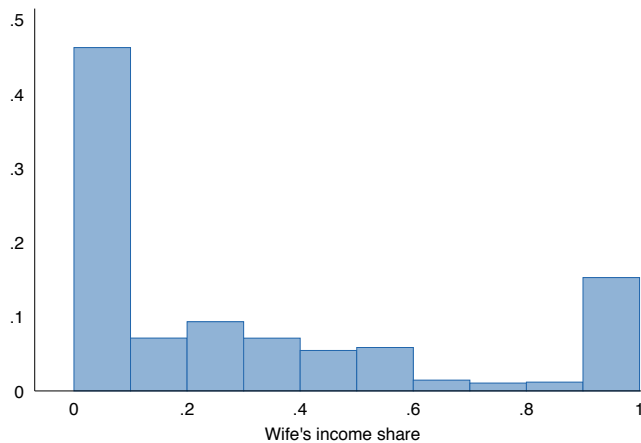
Figure D7: Distribution of wife's income share
